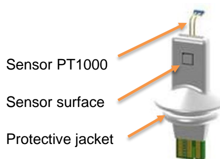
Figure 5: Hygro-thermo Measuring Element
