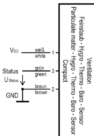
Figure 3: Connection of the status output
