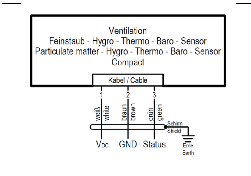
Figure 2: Ventilation connection diagram
